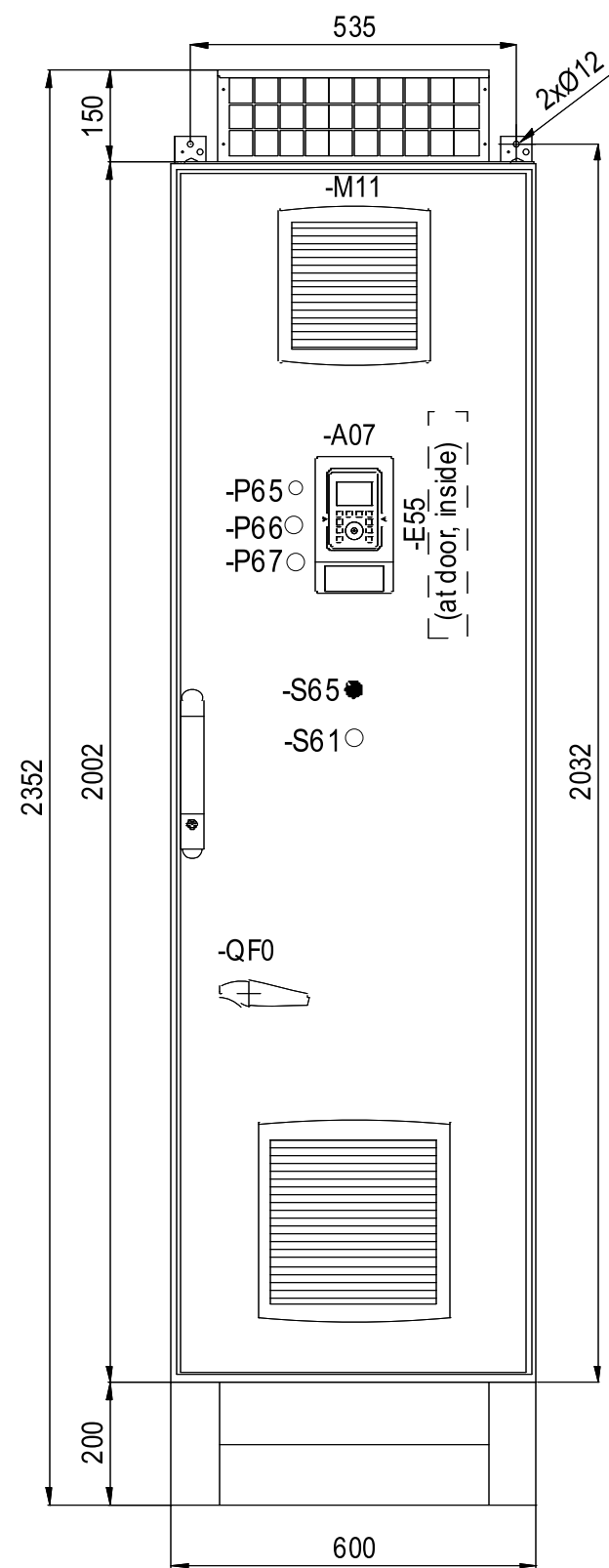
IP23 - Filters and Fan-Filter-Units without Filter Mats
